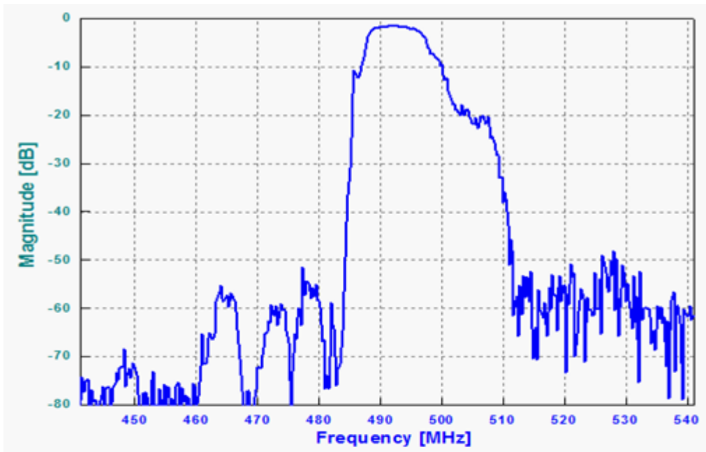
Frequency Response
